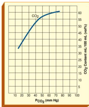
Fig. 7-3. Carbon dioxide dissociation curve.
