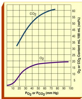
Fig. 7-6. Comparison of the oxygen and carbon dioxide dissociation curves in terms of partial pressure, content, and shape.
