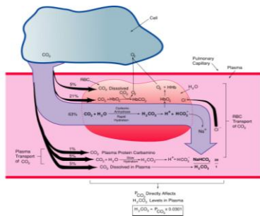
Fig. 7-1. How \text{CO}_2 is converted to \text{HCO}_3^- at the tissue sites. Most of the \text{CO}_2 that is produced at the tissue cells is carried to the lungs in the form of \text{HCO}_3^- .
