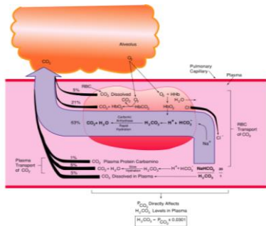
Fig. 7-2. How \text{HCO}_3^- is transformed back into \text{CO}_2 and eliminated in the alveoli.
