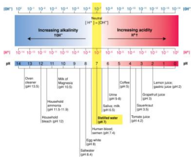
Figure 7-7 The pH values of representative substances. The pH scale represents the number of hydrogen ions in a substance. The concentration of hydrogen ions (H + ) and the corresponding hydroxyl concentration (OH - ) for each representative substance is also provided. Note that when the pH is 7.0, the amount of H + and OH - are equal and the solution is neutral.
