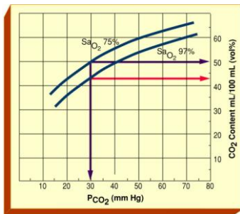
Fig. 7-5. Carbon dioxide dissociation curve at two different oxygen/hemoglobin saturation levels (SaO 2 of 97% and 75%). When the saturation of O 2 increases in the blood, the CO 2 content decreases at any given PCO 2 . This is known as the Haldane effect.
