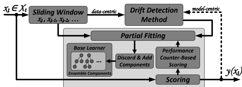
Figure 1. The workflow of PCB-iForest’s incremental learning framework.
