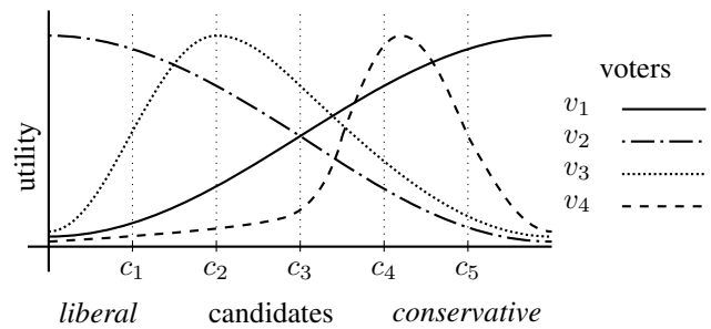
Figure 1: Example of a single-peaked electorate of four voters
