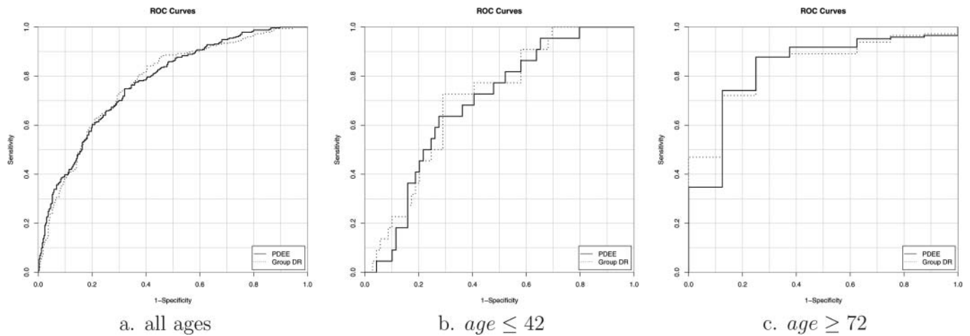
Figure 1. NHANES data: receiver operating characteristic curves for the derived composite biomarkers from PDEE and Group DR.
