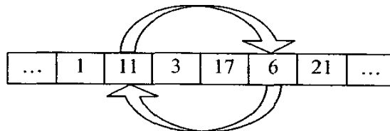
Figure 3: Particle mutation
