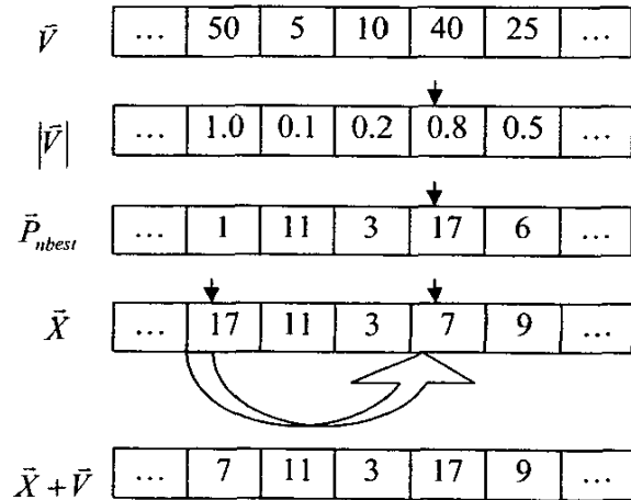
Figure 2: Particle update
