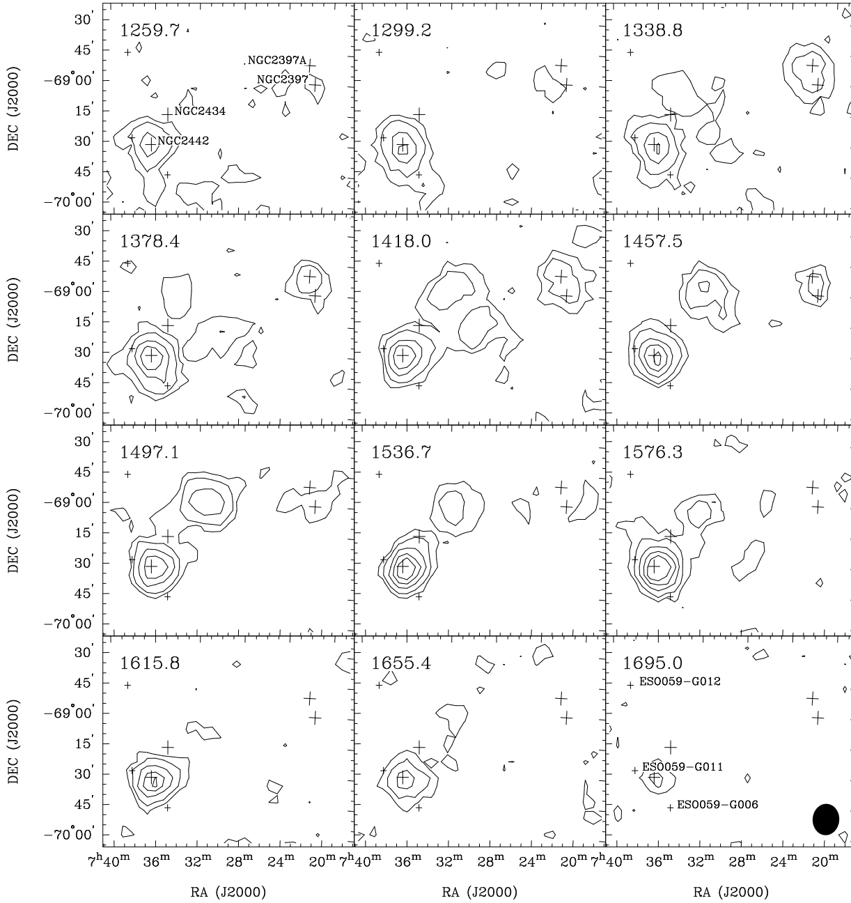
FIG. 4.— Channel maps of H I emission from the HIPASS observations of the region around NGC 2442. The contours correspond to flux densities of 15, 30, 60, 90, and 120 mJy beam -1 . For reference, the optical positions of the four major NGC galaxies in the field are marked in each panel with a large cross, and identified in the first panel; three more ESO galaxies are marked with small crosses, and identified in the last panel. The HIPASS beamsize is also indicated in the last panel.
