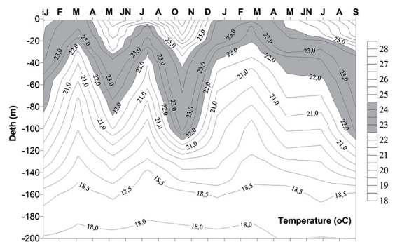
Figure 3. Distribution of temperature (°C) at the sampling station in Cariaco Basin from January 2006 to September 2007. Gray contours show the variability in the 23°C isotherm during coastal upwelling.
