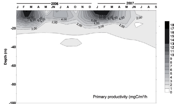
Figure 2. Distribution of primary productivity (mg C m-3 h-1) at the sampling station in Cariaco Basin from January 2006 to September 2007.
