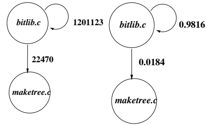
Figure 4. Execution counts and branching probabilities for bitlib.c
