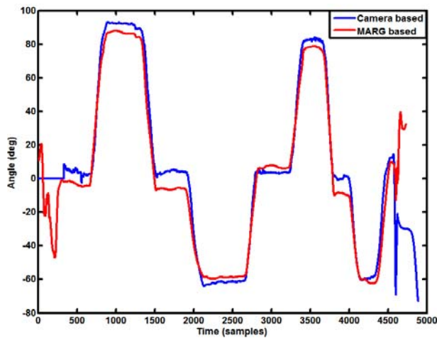
Fig. 7: Comparison of shoulder medial – lateral rotation angles
