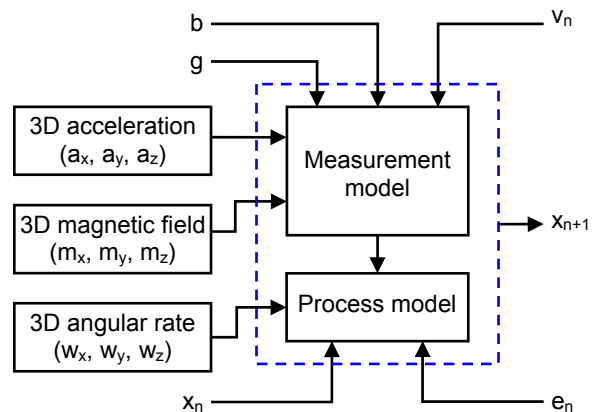
Fig. 2: Process diagram of data fusion algorithm.
