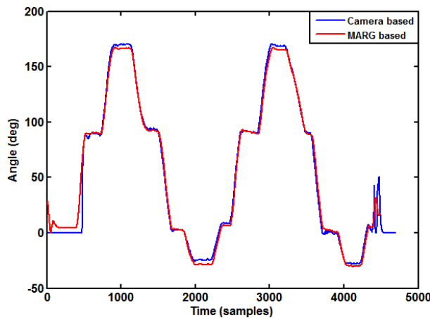
Fig. 5: Comparison of shoulder flexion – extension angles.
