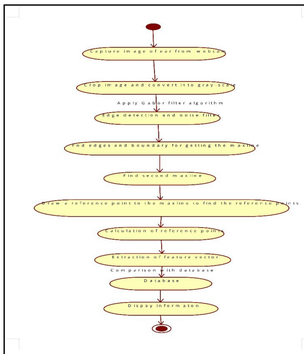
Fig. 2 Activity Diagram
