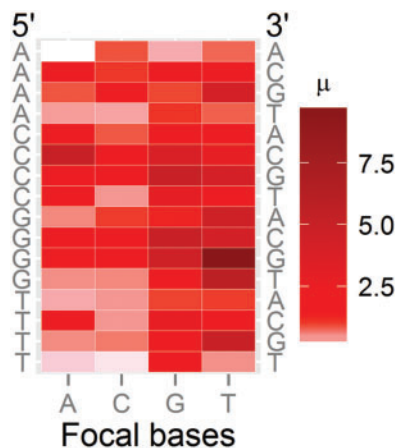
FIG. 4. —Context-dependent mutation rates. The heat map shows the mutation rates of each nucleotide context (5'-flanking nucleotide shown on the left, the focal bases at the bottom, and the 3'-flanking nucleotide on the right). \mu on the scale is the base-substitution mutation rate of the focal base given a specific nucleotide context on the leading strands; numbers on the scale are in the unit of 10^{-8} per site per generation.
