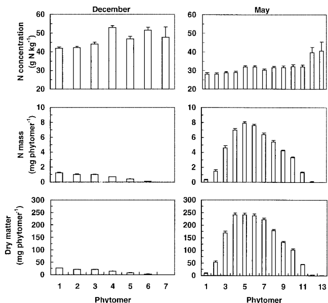
Fig. 4. Nitrogen concentration, N mass, and dry matter by phytomer (two-season means over all tissues and culms) with standard error bars.
