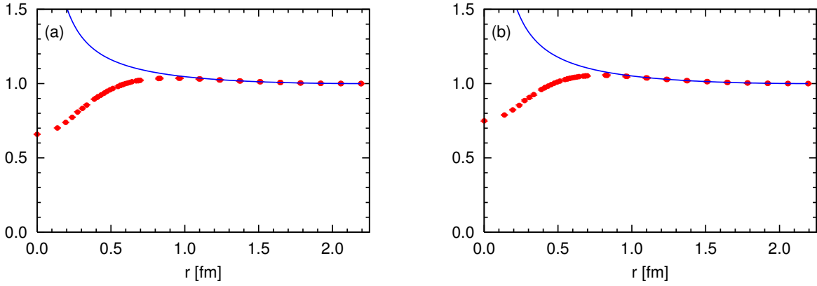
Fig. 2. (a) The fit of the NN wave functions for m_\pi = 529 MeV in the ^1S_0 channel using the Green's function in the fit range 11 \leq r/a \leq 16 . (b) Similar fit for the NN wave functions in the ^3S_1 channel.
