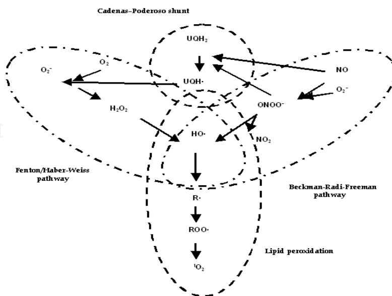
Figure 3. The free-radical mediated chain reaction in biochemistry. O_2^- , superoxide radical; H_2O_2 , hydrogen peroxide; HO\cdot , hydroxyl radical; NO, nitric oxide; ONOO^- , peroxynitrite; \cdot NO_2 , nitrogen dioxide; UQH 2 , ubiquinol; UQH \cdot , ubisemiquinone; R \cdot , alkyl radical; ROO\cdot , peroxy radical; ^1O_2 , singlet oxygen.
