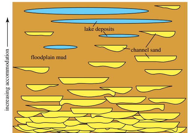
Figure 3. Idealized cross section, showing the change in architecture of terrestrial (river channel, floodplain, lake) deposits as the rate of accommodation increases. Adapted from [9].
