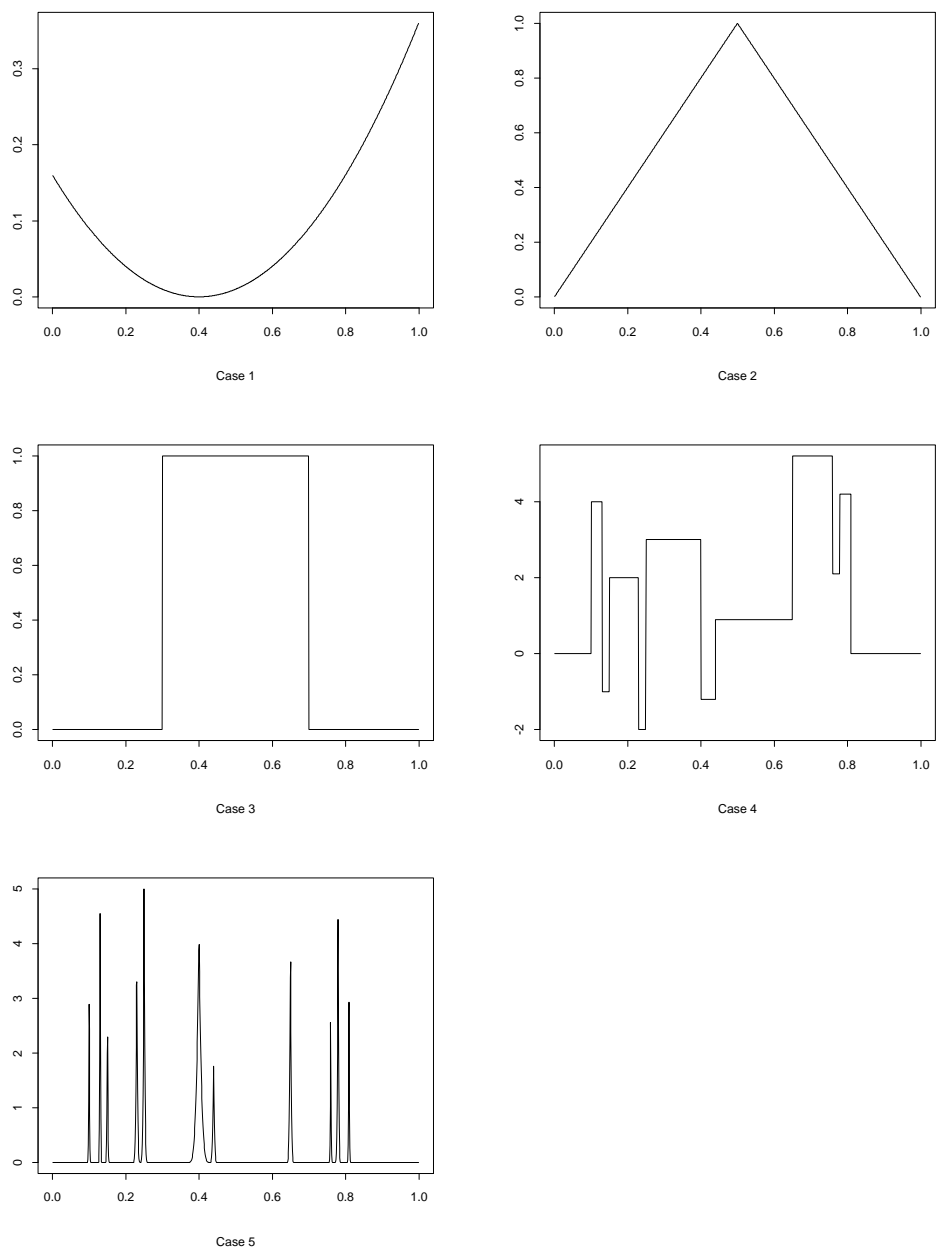
Fig. 2. Test-cases
