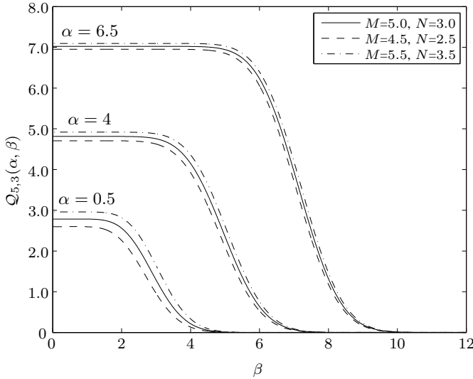
(a) Q_{5,3}(\alpha, \beta) versus \beta for several values of \alpha .
