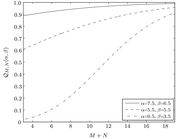
(a) \mathcal{Q}_{M,N}(\alpha, \beta) versus M + N for M - N = 1 .
