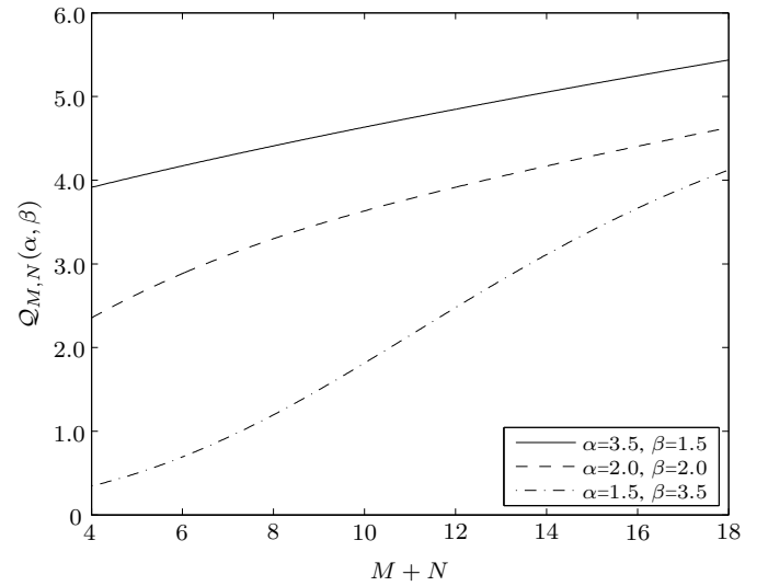
(b) \mathcal{Q}_{M,N}(\alpha, \beta) versus M + N for M - N = 2 .
