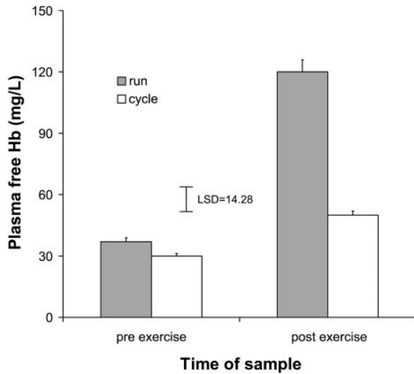
Fig. 2. Comparison of plasma free hemoglobin (in mg/l) before and after running and cycling for 1 h at 75% \dot{V}O_{2peak} . Values are means \pm SE; n = 10 subjects. Least significant difference (LSD) is equivalent to twice the SE of the differences. Any pair of means differing by more than the LSD is significantly different at P = 0.05 .
