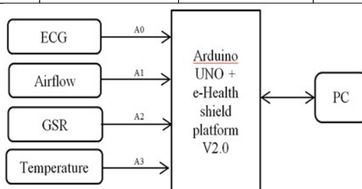
Figure 6. Show the block diagram for e-Health monitoring design.
