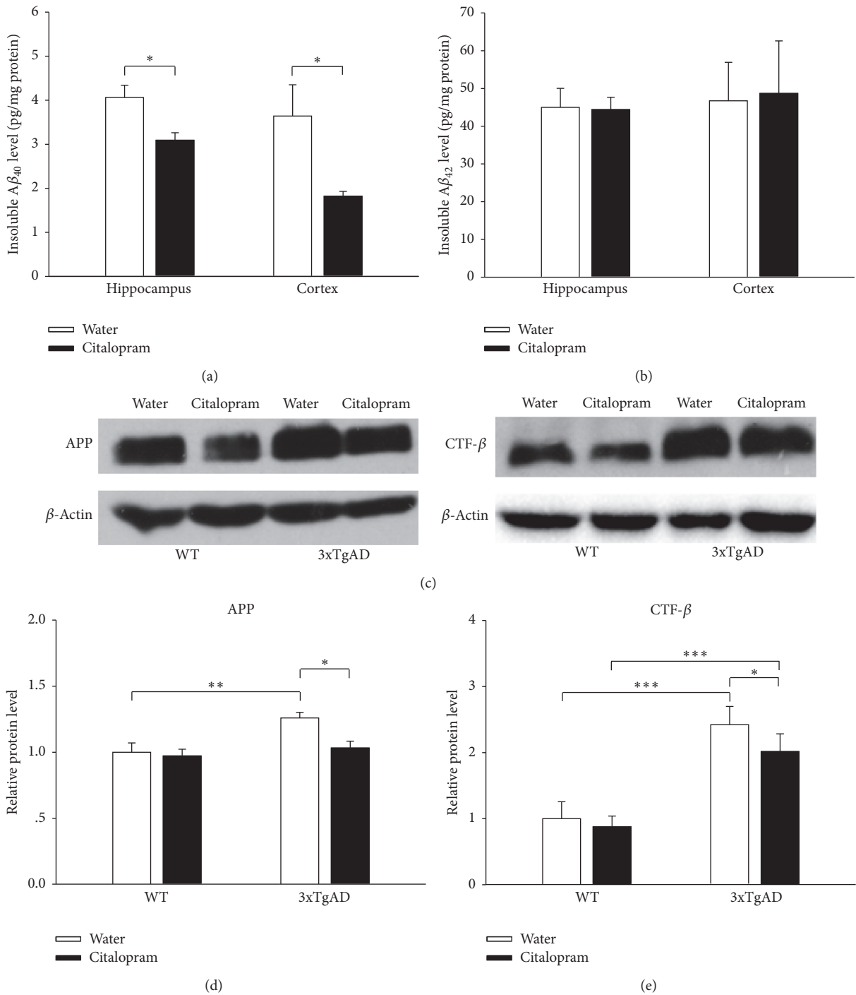
FIGURE 5: Citalopram treatment decreased A \beta production by inhibiting APP expression in 3xTgAD mice. (a) The insoluble A \beta_{40} concentrations in the hippocampus and cerebral cortex samples from citalopram-treated 3xTgAD mice were significantly lower than the concentrations in water-treated 3xTgAD mice. (b) Citalopram treatment did not have significant effect on the levels of insoluble A \beta_{42} in the hippocampus and cerebral cortex. (c) Representative western blot images of APP and CTF \beta in different groups. (d) Citalopram treatment downregulated APP expression in 3xTgAD mice. (e) Citalopram treatment decreased CTF \beta levels in 3xTgAD mice. Error bars indicate SEM. * P < 0.05 , ** P < 0.01 , and *** P < 0.001 .
