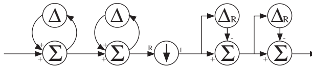
Fig. 12. Flat SDF model of CIC decimator.
