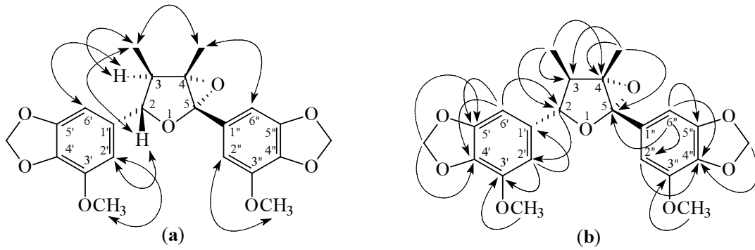
Fig. 2S Significant NOESY (a) and HMBC (b) correlations of 3.
