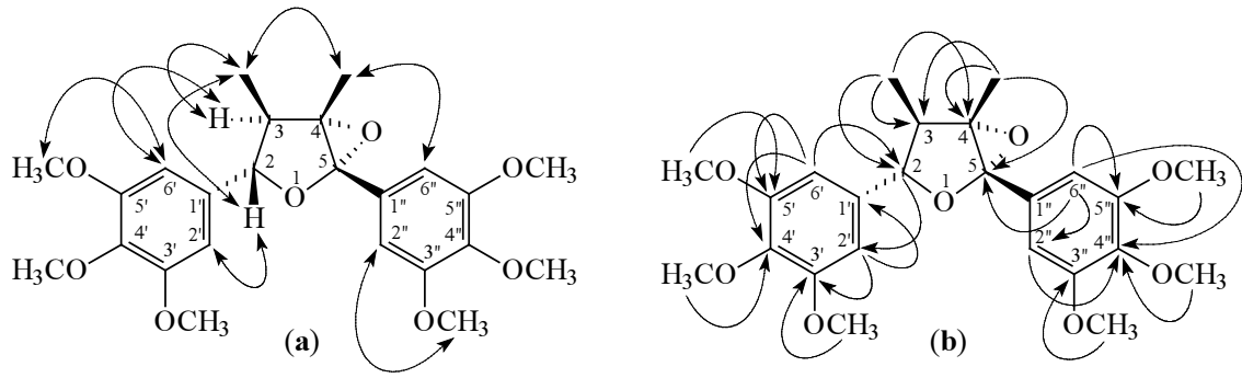
Fig. 1S Significant NOESY (a) and HMBC (b) correlations of 2.
