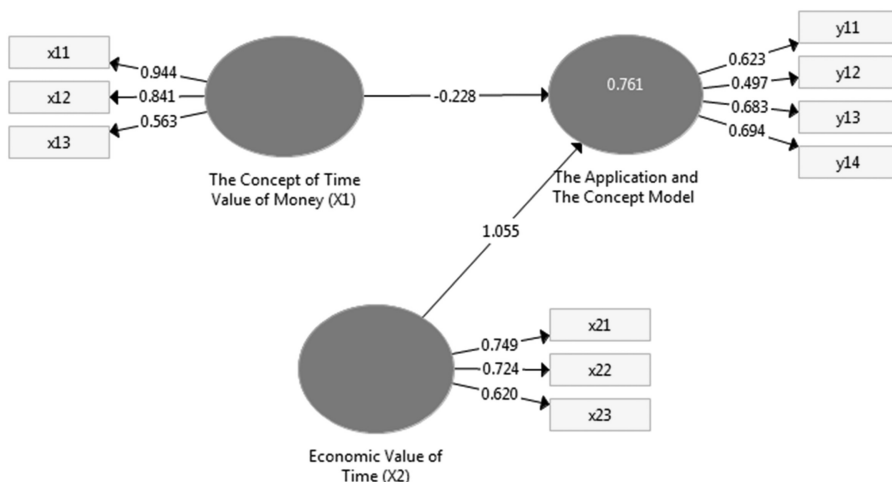
Figure 1. Overall Model with Coefficient
