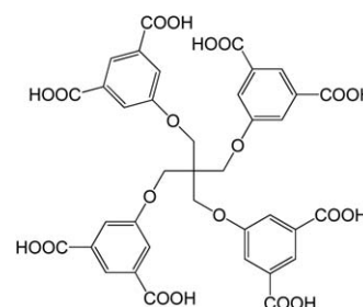
Scheme 1 Schematic structure of H_8L .
