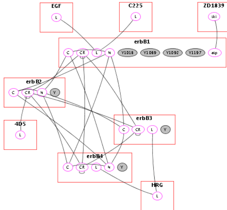
Fig. 4. Contact map of the consensus model with antibodies (C225 and 4D5) as competitive inhibitors, and ZD1839 as non-competitive inhibitor.
