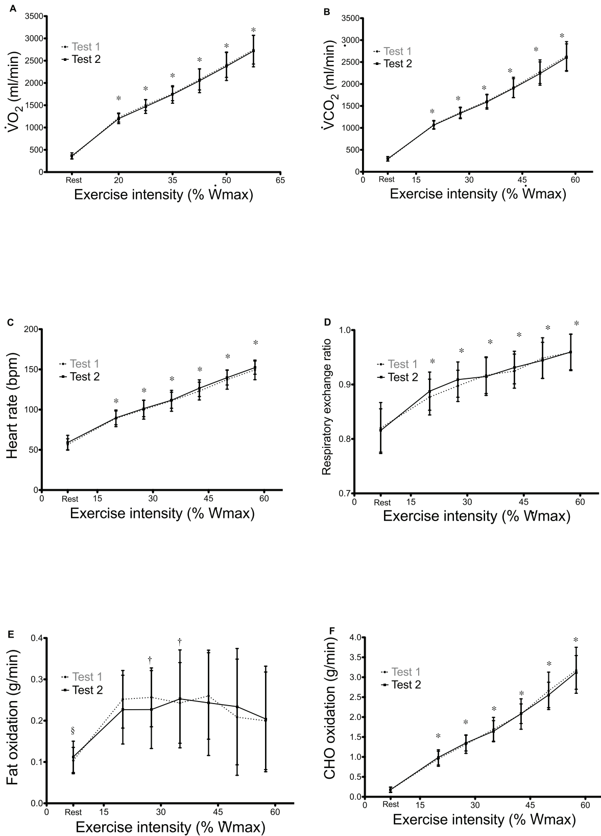
Figure 2. Course of average \dot{V}O_2 , \dot{V}CO_2 , HR, RER, F_{ox} and CHO_{ox} during two identical submaximal incremental tests (mean and SD). \dot{W}_{umax} , maximal aerobic power output; \dot{V}O_2 , oxygen uptake; \dot{V}CO_2 , carbon dioxide production; RER, respiratory exchange ratio; HR, heart rate; F_{ox} , fat oxidation rate; CHO_{ox} , carbohydrate oxidation rate. *significantly increases with exercise intensity, §rest significantly different than exercise (20–57.5% \dot{W}_{umax} ), † significantly different than 57.5% \dot{W}_{umax} . doi:10.1371/journal.pone.0097930.g002
