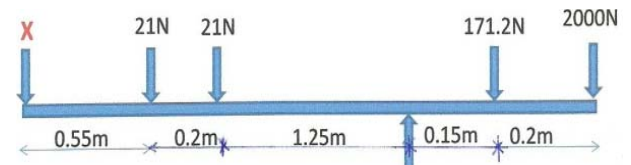
Fig. 12: Free body diagram of the main frame
