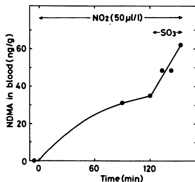
FIGURE 4. Accelerating effect of \text{SO}_3 on NDMA formation in a rabbit (2.2 kg) administered aminopyrine IV and 50 \mu\text{L/L} \text{NO}_2 by inhalation. \text{SO}_3 was added by passing the gas (2 L/min) over a solution (0.3 mL) of 60% fuming sulfuric acid. Aminopyrine was administered as described in Fig. 3.
