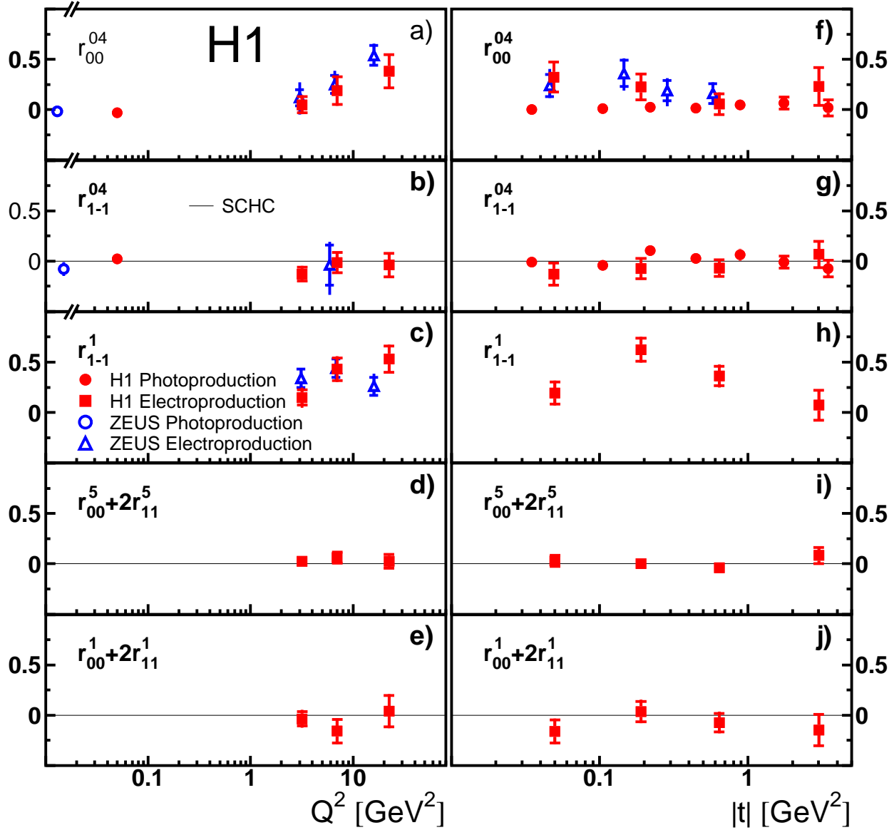
Figure 12: Spin-density matrix elements as functions of Q^2 (a-e) and |t| (f-j) for the range 40 < W_{\gamma p} < 160 GeV. The data points are the results of fits of equations 4- 7 to the data shown in figure 11. The inner error bars show the fit result including only the statistical error, while the outer error bars also include the systematic uncertainties. The expectations from SCHC are shown as solid lines. The results from the ZEUS collaboration are also shown, ( a), c) and f) [6, 16] and b) [5, 15]).
