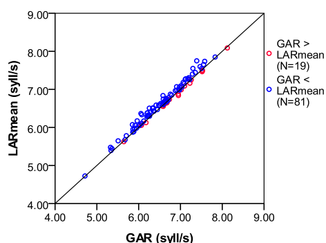
Figure 4: Scatterplot for GAR and LARmean values.
