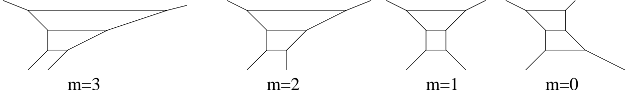
Figure 8: Splitting local \mathbb{F}_m into K_{R_i R_j}^{(m)} contributions.
