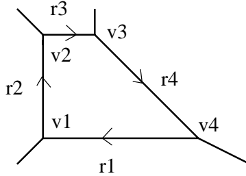
Figure 4: Web diagram of local \mathbb{P}^2 blown up at one point.
