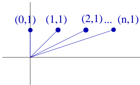
Figure 14: The resolved A_{n-1} geometry.
