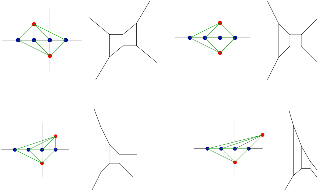
Figure 16: A_2 fibrations over \mathbb{P}^1 .
