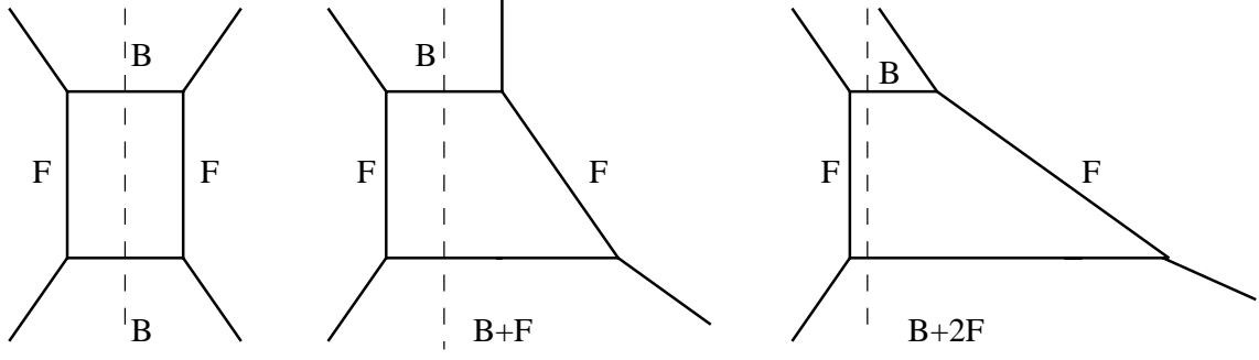
Figure 8: Splitting local \mathbb{F}_m into K_{R_i R_j}^{(m)} contributions.
