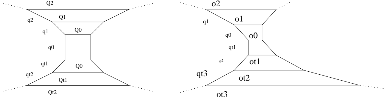
Figure 12: Identifying the Kähler classes of curves, for geometries containing even Hirzebruch surfaces (left), and odd (right).
