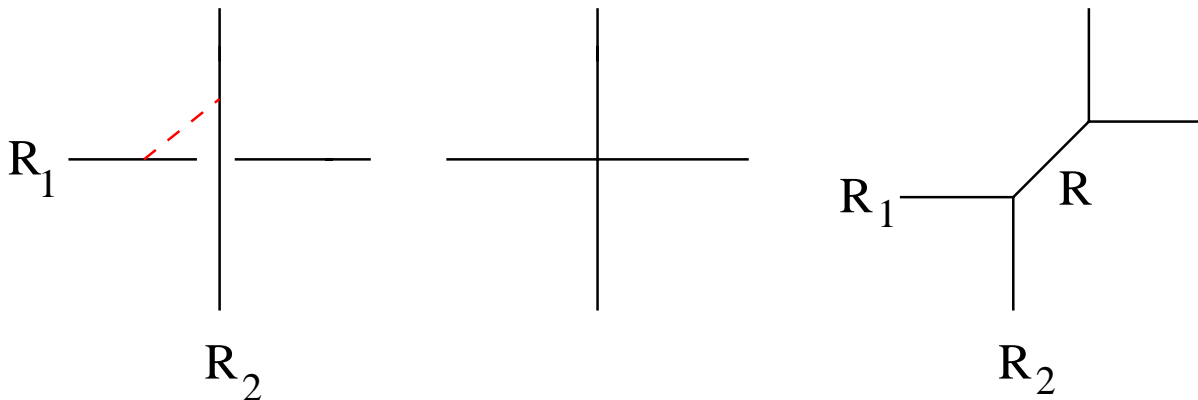
Figure 7: A local transition.
