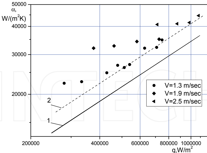
Fig. 13. Dependence of the heat transfer factor \alpha on the heat flux q at water boiling (pressure p=0.14 MPa) in a tube with roughness shown in fig. 2, a: 1 - heat transfer at pool boiling on smooth wall (by calculation); 2 - heat transfer at pool boiling on rough wall
