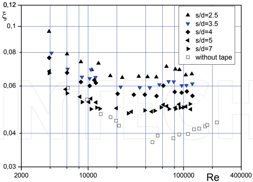
Fig. 25. Dependence of hydraulic resistance factor of rough tubes with rectangular roughness profile (Table 2, № 5) on Re at various S/d
