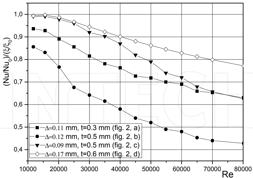
Fig. 5. Thermohydraulic efficiency of rough tubes
