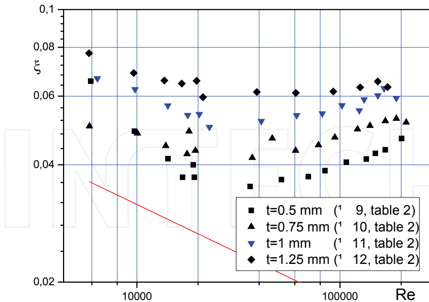
Fig. 17. Dependence of hydraulic resistance factor of rough tubes with rounded thread roughness profile on Re : line – for smooth tube (by calculation)
