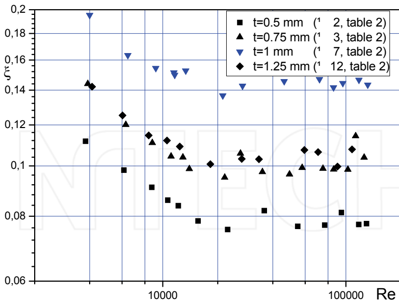
Fig. 24. Dependence of hydraulic resistance factor of rough tubes with various thread roughness profile with similar heights of ledges and with twisted tape insert ( S/d=2.5 ) on Re
