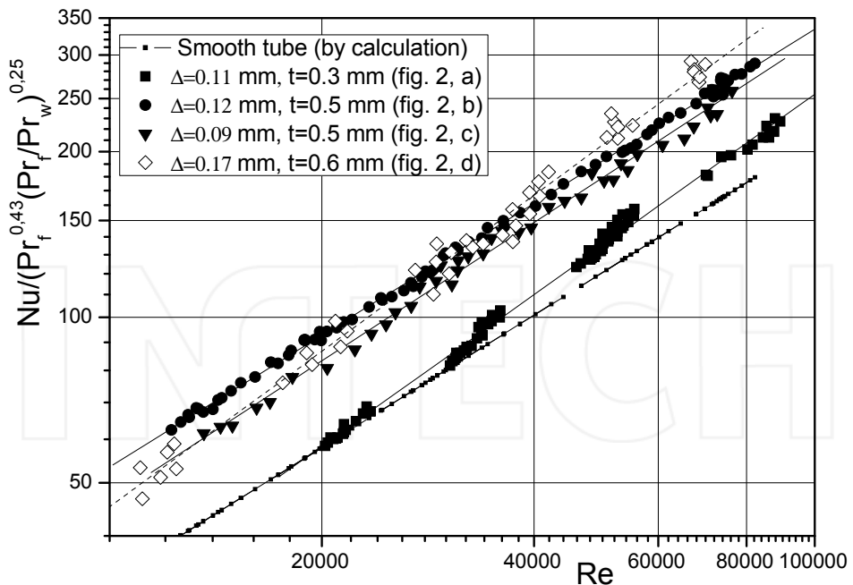
Fig. 3. Dependence of dimensionless heat transfer of rough tubes on Re
