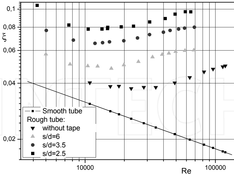
Fig. 12. Hydraulic resistance of tubes with a uniform continuous roughness (with profile shown in fig.2, c) and with an inserted twisted tape
