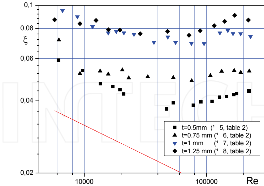
Fig. 16. Dependence of hydraulic resistance factor of rough tubes with rectangular thread roughness profile on Re : line – for smooth tube (by calculation)
