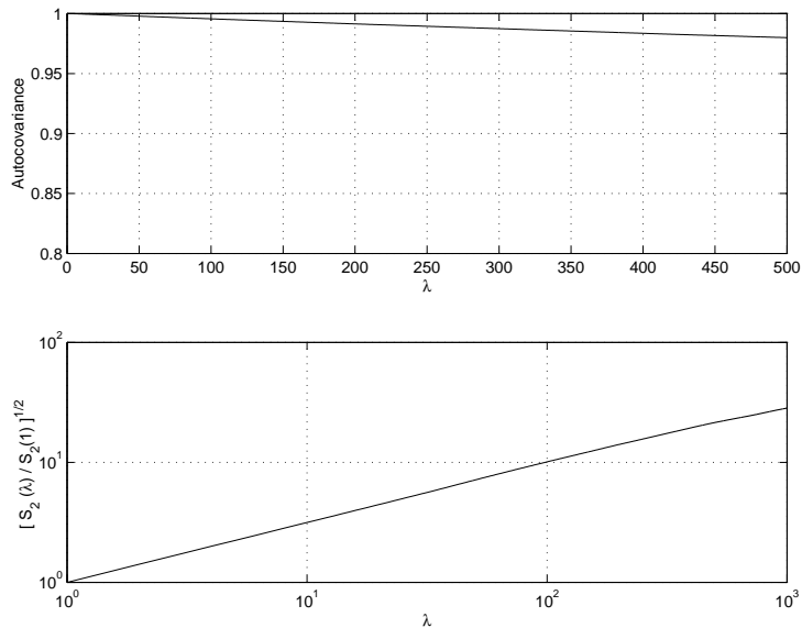
Figure 2: Autocovariance (top panel) and scaling plot (bottom panel) for model Brownian motion ( H = 0.5 ).
