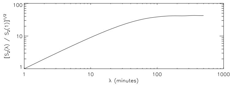
Figure 5: Scaling plot for random Weimer pulse train.
