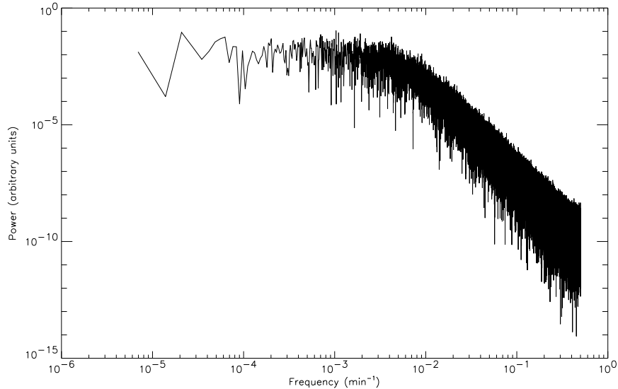
Figure 3: Representative example of a spectrum from a random Weimer pulse train.
