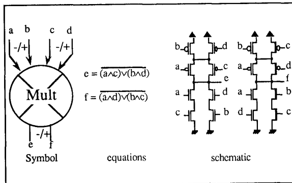
Fig. 5 Elementary SBD multiplier.
