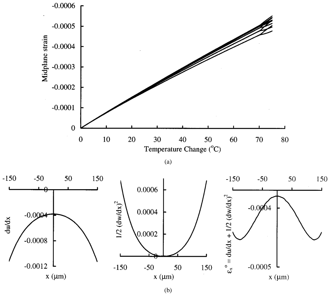
Fig. 13. (a) Pointwise midplane strain \varepsilon_x^0 (and \varepsilon_y^0 ) at five locations 2x/L (and 2y/L ) as a function of temperature change for the L = 300 \mu\text{m} microstructure. Curves before bifurcation correspond to 2x(2y)/L = 0.67, 0.83, 0.5, 0.33, and 1 from top to bottom; (b) Midplane strain for the L = 300 \mu\text{m} microstructure and its components du/dx , and (1/2)(dw/dx)^2 along y = 0 for \Delta T = -76 \text{ }^\circ\text{C} .
