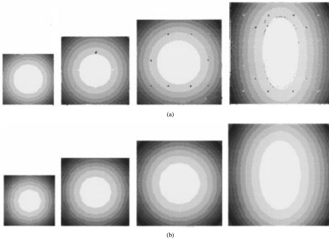
Fig. 4. Contour plots of the (a) measured, and (b) predicted transverse displacements w(x, y) at room temperature for the four gold-polysilicon square plates: L = 150, 200, 250, and 300 \mu\text{m} from left to right. Each contour band represents a displacement of 0.23, 0.35, 0.45, and 0.6 \mu\text{m} for the L = 150, 200, 250, and 300 \mu\text{m} plates, respectively.
