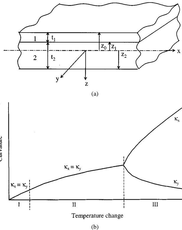
Fig. 1. Schematic of (a) the geometry of the two-layer plate microstructure showing relevant dimensions, and (b) the general characteristics of the average curvature versus temperature change of a two-layer plate microstructure.
