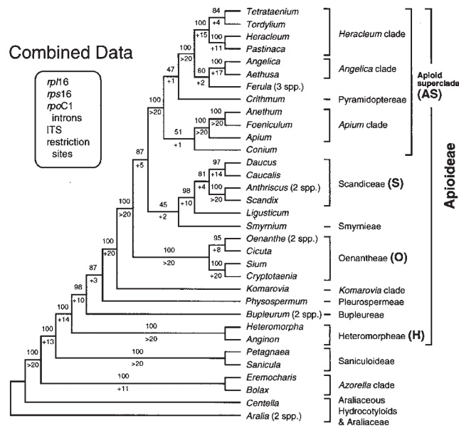
FIG. 3. Single minimal length 3929-step tree derived from maximum parsimony analysis of combined DNA sequence ( rpl16 intron, rps16 intron, rpoC1 intron, ITS) and restriction site data (CI, excluding uninformative characters = 0.482; RI = 0.639). Numbers above nodes are bootstrap estimates for 1000 replicate analyses; numbers below nodes are decay values for trees up to 20 steps longer than those most parsimonious. The Ferula , Anthriscus , Oenanthe , Bupleurum and Aralia species examined in each of the separate analyses were not identical; however, because each group of species is monophyletic (as revealed by our earlier, more comprehensive analyses), data for each genus were combined and treated as a single exemplar. Data for genera not included in any separate analysis were scored as missing data. Complete species names are indicated in Table 5. The bracketed tribes and clades are those listed in Tables 2 and 3; the abbreviations AS, S, O and H are the same as outlined in Fig. 2.
