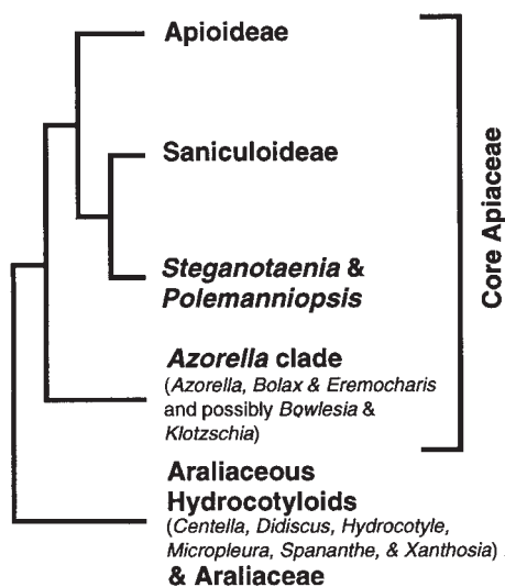
FIG. 1. Summary of relationships within core Apiaceae as revealed by phylogenetic analyses of molecular data (Plunkett et al. , 1996a, 1997; Downie & Katz-Downie, 1999; Downie et al. , 1998, 2000b). Members of the Azorella clade and the araliaceous hydrocotyloids ( Didiscus DC. ex Hook. = Trachymene Rudge) are treated by Pimenov & Leonov (1993) in Apiaceae subfamily Hydrocotyloideae ; the araliaceous hydrocotyloids do not comprise a monophyletic group (Plunkett et al. , 1997; Downie & Katz-Downie, 1999; Downie et al. , 2000b). Steganotaenia and Polemanniopsis ( Apiioideae and incertae sedis , respectively; Pimenov & Leonov, 1993), form a clade sister to Saniculoideae and, pending further study, may belong within this subfamily (Downie & Katz-Downie, 1999).
