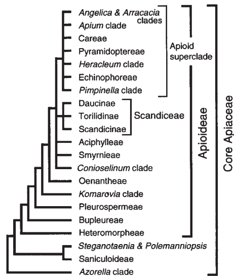
FIG. 5. Summary of relationships among the tribes (Table 2) and informally recognized clades (Table 3) of Apiaceae subfamily Apioideae as revealed by phylogenetic analyses of molecular data (this study; Downie & Katz-Downie, 1999; Downie et al. , 1998, 2000a,b,c). Not all genera examined to date have been assigned to a particular group (Table 4); many of these genera, however, are contained within the apioid superclade.
