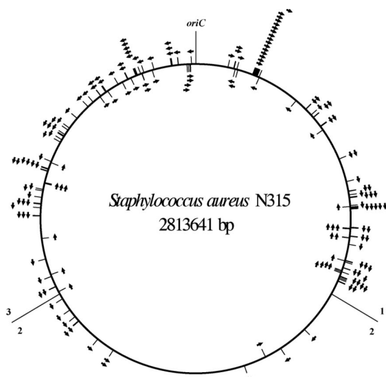
FIG. 2. Chromosomal distribution and orientation of ORFs up-regulated by \sigma^B . ORFs and their respective orientations are represented by arrows. The origin of replication ( oriC ) and the borders of genome fragments 1 to 3 are indicated.
