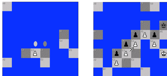
Figure 5. States 11 and 55 of an execution of Capablanca. There is fast convergence to the most important areas of the board: At state 55, all pieces but the bishop have been registered (as has a first defense relation).
