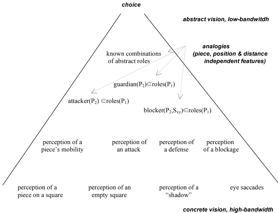
Figure 2. The emergence of choice: as time progresses, humans move (in a non-monotonic way) from higher-bandwidth to lower bandwidth processes; from concrete observations to abstract observations. Note that there are multiple levels of perceptions involved, and interpretations will be construed by, and bind, these perceptions in all levels. From the particular pieces to the (important or irrelevant) roles these pieces are playing, a final representation should encompass information from these multiple levels. Note finally that information may flow through all of these processes, vertically and horizontally: a glance at a “shadow” (see below) can lead to the perception of a particular piece; perception of a particular piece can lead to the perception of an attack; and perception of an attack can lead to the top-down, hypothesis-driven, search for a piece capable of blocking such attack.
