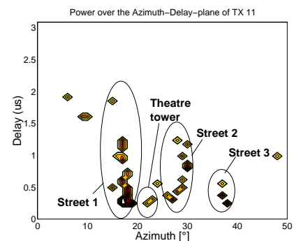
Fig. 9. TX11: Azimuth-delay
