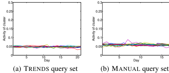
Figure 5: Temporal profile of latent clusters given by TENSORCOMPARE, for Google and Bing. The y -axis corresponds to the membership of the particular day to the cluster of interest. For both query sets, the temporal profile of all clusters is approximately constant over time. In particular, each value for TRENDS is \approx 1/21 and for MANUAL it is \approx 1/17 . As stated in Section 3.1, this indicates that both Bing and Google returned persistent results, at least during the duration of our experiment. Due to this uniformity, we overplot all clusters, without making any distinctions.
