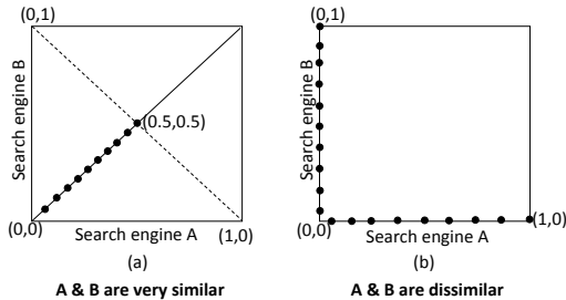
Figure 1: Visualization guide for TENSORCOMPARE.
