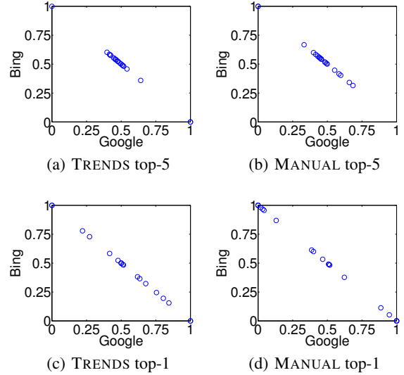
Figure 8: TENSORCOMPARE sensitivity
