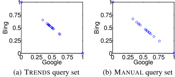
Figure 4: Visualization of TENSORCOMPARE for Google and Bing. Values on the x -axis correspond to the membership of Google to a cluster, and values on the y -axis correspond to the membership of Bing. Thus, an (x, y) point on this plot represents one of the clusters of TENSORCOMPARE. The closer the points are to the 45-degree line, the more similar are the two search engines.
