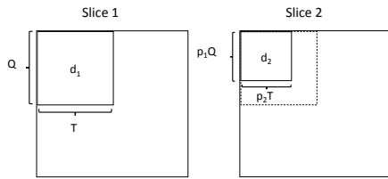
Figure 10: The two slices of \underline{X} .
