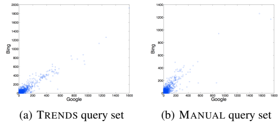
Figure 3: Term distribution between Google and Bing search results.
