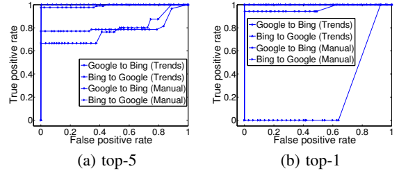
Figure 9: CROSSLearnCOMPARE sensitivity
