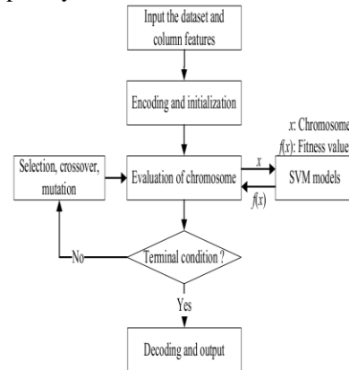
Fig 2.1 Process Flow Diagram of GA-SVM algorithm
