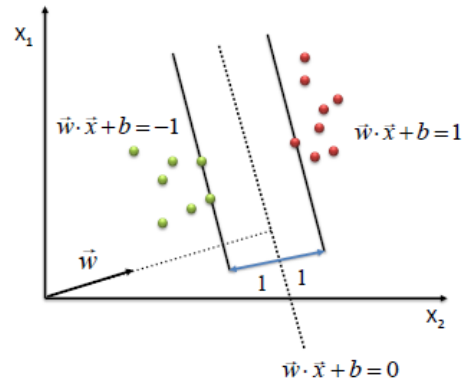
Figure 5.1: Support vector machine
