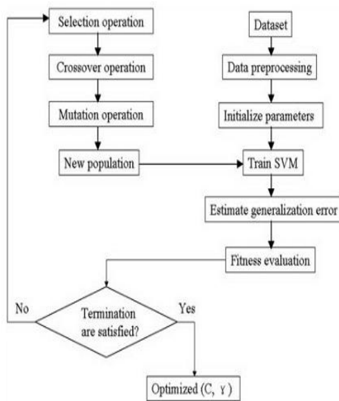
Fig 2.2 Flow Chart of GA-Based Parameter Optimization
