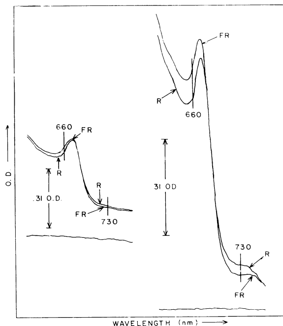
FIG. 1. In vivo absorption spectra of embryos 16 hr from start of soaking of the seeds. Left: before adding water; right: after adding water. The red (R) and far-red (FR) irradiations were 2 min saturating dosages.
