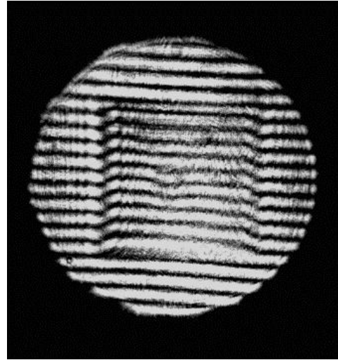
Figure 5. An interferogram of a 1-cm InGaAs transmissive MQW modulator is shown. The ripples around the square are edge effects around the sample. It can be seen that the surface is relatively good and should not deleteriously impact system performance.
