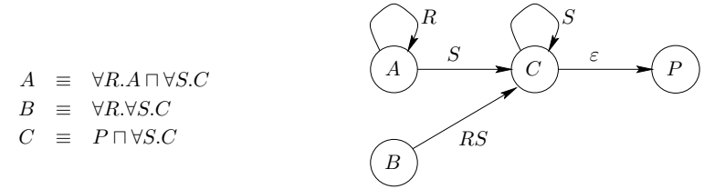
Fig. 2.7. A TBox and the corresponding automaton.
