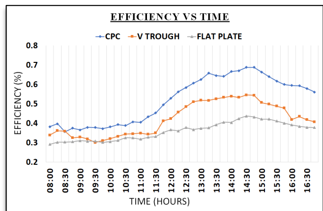
Figure 18. Efficiency vs Time values observed for the Flat plate, V Trough and CPC Collector
