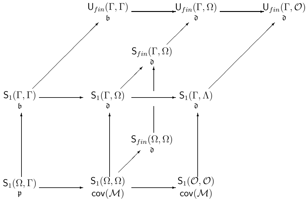
Figure 4: Cardinals \text{non}(P)
