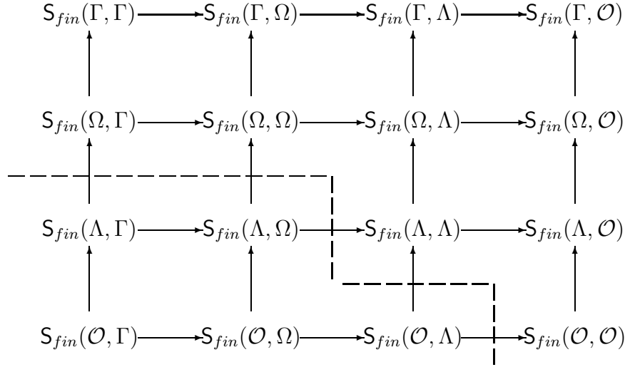
Figure 1: Basic diagram for S_{fin}
