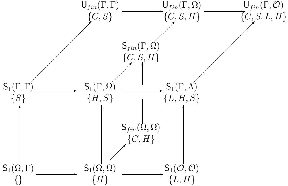
Figure 3: After removing equivalent classes
