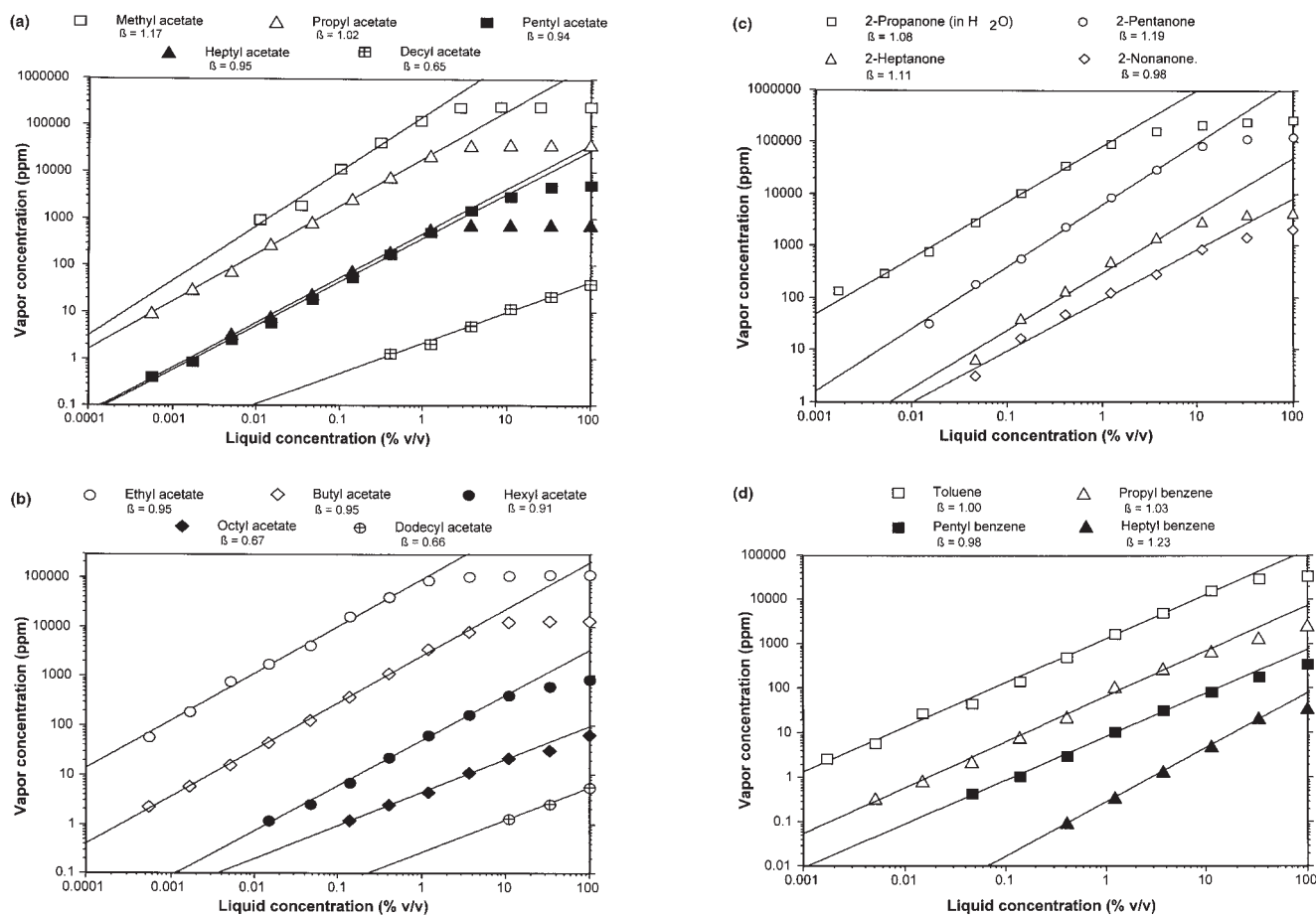
Figure 2 Analogous to Figure 1, but for homologous acetate esters (a,b), 2-ketones (c), alkylbenzenes (d,e), aliphatic aldehydes (f) and carboxylic acids (g).
