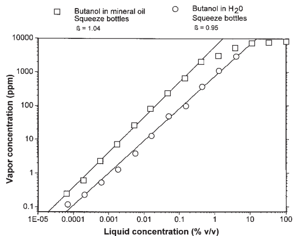
Figure 3 Vapor (p.p.m. by volume) vs. liquid (% v/v) concentration for 1-butanol with either mineral oil or distilled water as solvent. The slope ( \beta ) of the fitted function is shown.
