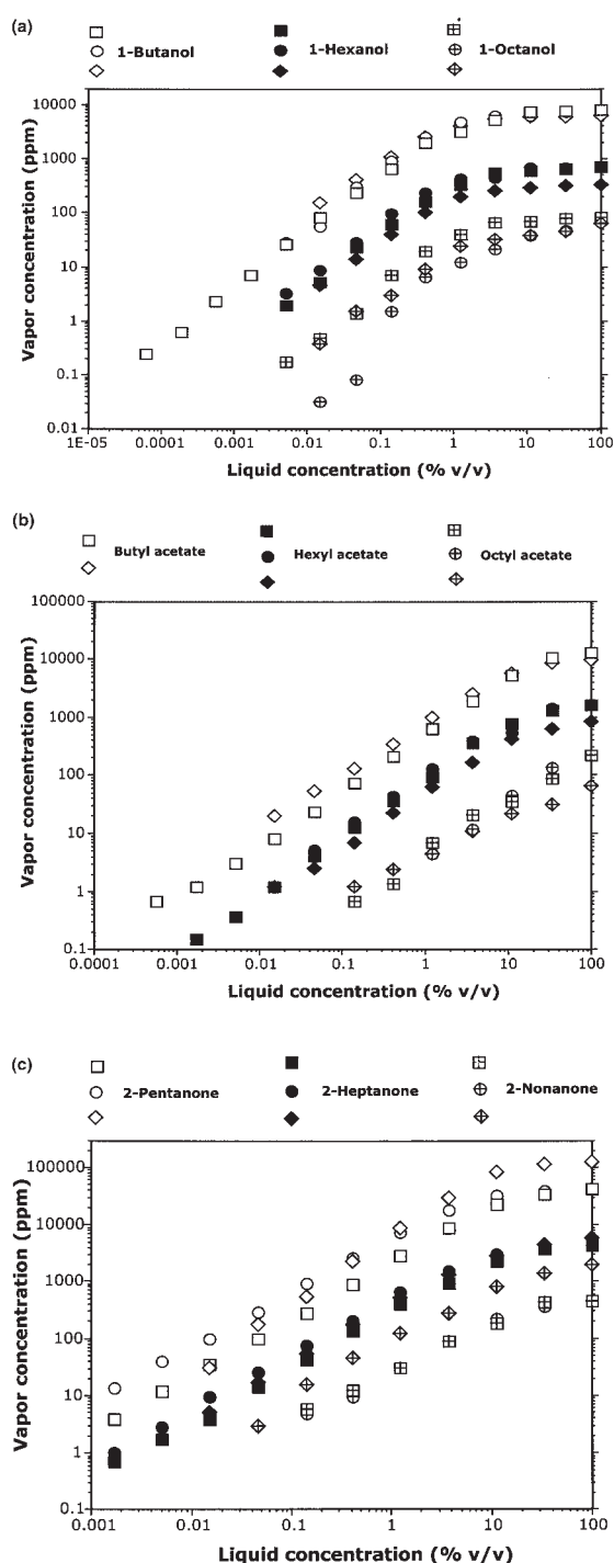
Figure 6 Showing the stability of relationships of vapor (p.p.m. by volume) vs. liquid (% v/v) concentration for three homologous n-alcohols (a), acetate esters (b) and 2-ketones (c), under different conditions (see text). For all panels, conditions include: using squeeze bottles re saturated vapor concentration (squares), using glass vessels re saturated vapor concentration (circles), and building a calibration curve for mass (diamonds).
