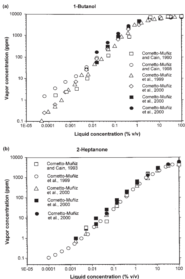
Figure 5 Showing the agreement among vapor concentrations of a VOC, produced by the same liquid dilution, measured across different studies through the years, involving different conditions in terms of: odor-delivery containers, calibration strategies, GC sampling techniques, use or not of pre-concentration methods, and presence or absence of other chemicals in the sample (see text). Panels (a-d) present the results for 1-butanol, 2-heptanone, butyl acetate and toluene, respectively.
