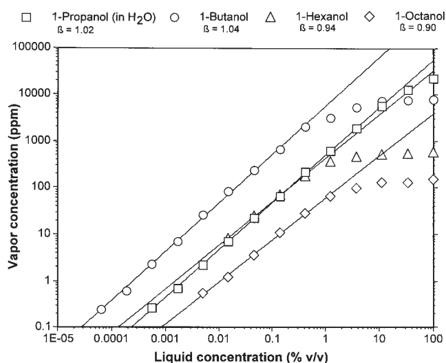
Figure 1 Vapor (p.p.m. by volume) vs. liquid (% v/v) concentration for homologous alcohols in logarithmic coordinates. Except where indicated, the solvent was mineral oil. The exponent \beta (slope in the double logarithmic coordinates of the figure) is indicated for each VOC. See Table 1 for the specific values and applicable concentration range of the power equation for each chemical.
