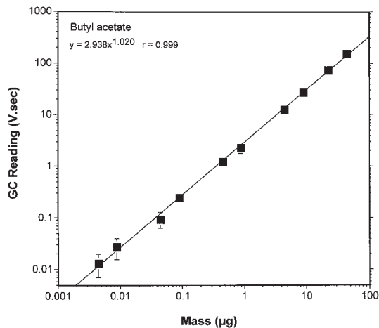
Figure 4 GC calibration curve for liquid-phase butyl acetate showing GC readings (V.sec) as a function of injected mass ( \mu\text{g} ). The equation of the curve is shown. Bars, sometimes hidden by the symbol, represent standard deviations.
