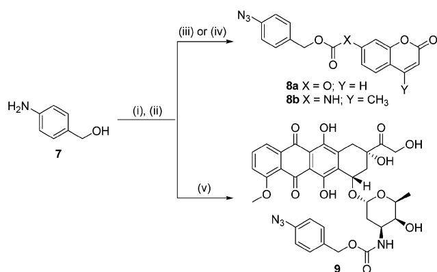
Scheme 2 Conditions: (i) NaNO 2 , 5 M HCl then NaN 3 , 0 °C, 73%; (ii) 4-nitrophenyl chloroformate, pyridine, DCM, 25 °C, 57%; (iii) 7-hydroxycoumarin, Et 3 N, DMF, 25 °C, 38%; (iv) 7-amino-4-methylcoumarin, triphosgene, toluene, reflux, then 4-azidobenzyl alcohol, 25 °C, 30%; (v) doxorubicin·HCl, Et 3 N, 4 Å molecular sieves, DMF, 25 °C, 69%.
