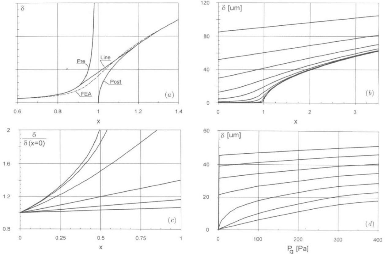
Figure 2. Mid-point deflections for the silicon beam in figure 1, with L = 10 mm, b = 1.2 mm, t = 34 \mu\text{m} and E = 167 GPa ((110)). The solid curves in figure 2(a) are based on equation (3a) with p_g = 10 Pa, while the other have been determined with FEA (ANSYS). The curves are, from top to bottom, for p_g = 10\text{k}, 3\text{k}, 1\text{k}, 300, 100, 30, 3 and 1 Pa (figure 2(b)), p_g = 30, 100, 300, 1\text{k}, 3\text{k} and 10\text{k} Pa (figure 2(c)) and T_g = 34, 29, 24, 19, 14, 9 and 4 °C (figure 2(d), T_c = 14.7 °C).
