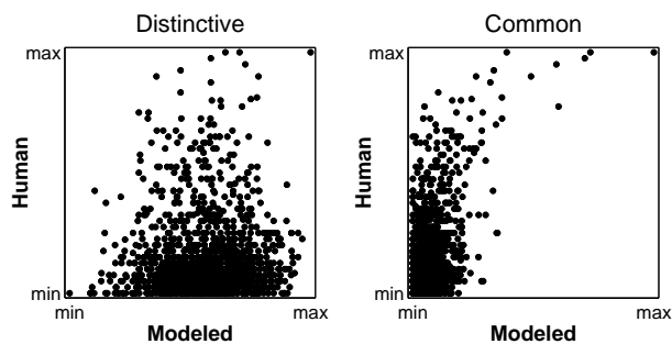
Figure 5: The relationship between model and human judgments of similarity for all document pairs, using the distinctive features (left panel) and the common features models (right panel), using the binary features representation based on 8-grams.
